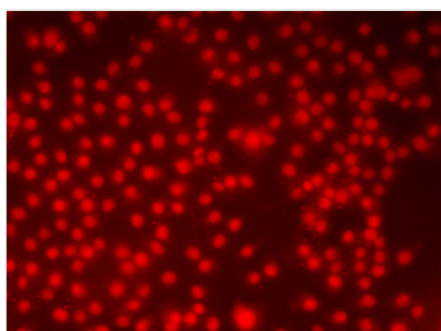
Immunofluorescent staining of HeLa cells showing nuclear staining with anti-HMGB1 antibody at a dilution of 1/100
