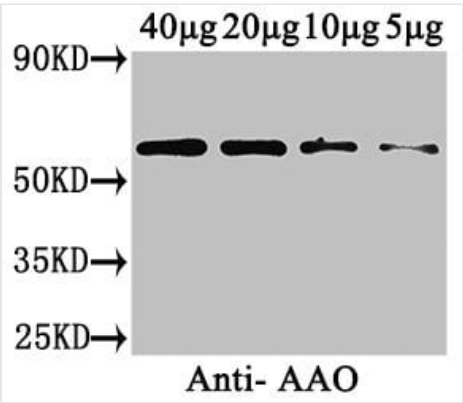
WB (Western Blot) Western BlotPositive WB detected in: Cucurbita maxima(40ug,20ug,10ug,5ug)All lanes: AAO antibody at 3ug/mlSecondaryGoat polyclonal to rabbit IgG at 1/50000 dilutionPredicted band size: 65 kDaObserved band size: 65 kDa
