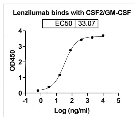
Bioactivity Detects Human CSF2/GM-CSF in direct ELISAs.
