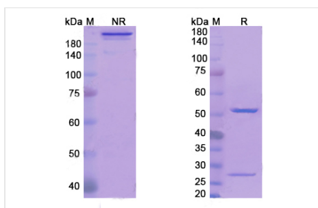
SDS-PAGE SDS PAGE for Avizakimab
