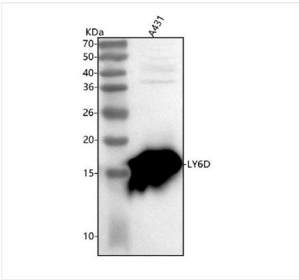
WB (Western Blot) Figure 1. Western blot analysis of LY6D using anti-LY6D antibody (AAA127604). Electrophoresis was performed on a 5-20% SDS-PAGE gel at 70V (Stacking gel)/90V (Resolving gel) for 2-3 hours. The sample well of each lane was loaded with 30 ug of sample under reducing conditions. Lane 1: human A431 whole cell lysates. After electrophoresis, proteins were transferred to a nitrocellulose membrane at 150 mA for 50-90 minutes. Blocked the membrane with 5% non-fat milk/TBS for 1.5 hour at RT. The membrane was incubated with rabbit anti-LY6D antigen affinity purified polyclonal antibody (#AAA127604) at 0.25ug/mL overnight at 4 degree C, then washed with TBS-0.1%Tween 3 times with 5 minutes each and probed with a goat anti-rabbit IgG-HRP secondary antibody at a dilution of 1:5000 for 1.5 hour at RT. The signal is developed using an Enhanced Chemiluminescent detection (ECL) kit with Tanon 5200 system. A specific band was detected for LY6D at approximately 16 kDa. The expected band size for LY6D is at 13 kDa.
