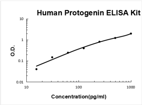
Standard Curve (Sample) Human Protogenin PicoKine ELISA Kit standard curve
