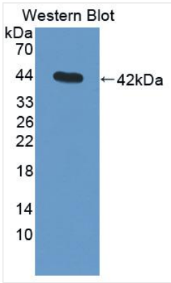
WB (Western Blot) Western Blot; Sample: Recombinant C3, Mouse.
