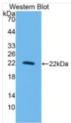
WB (Western Blot) Western Blot: Sample: Recombinant IL10, Rat.
