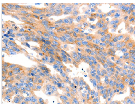
IHC (Immunohistochemistry) Immunohistochemistry of paraffin-embedded Human ovarian cancer using MAP2K2 Polyclonal Antibody at dilution of 1:100
