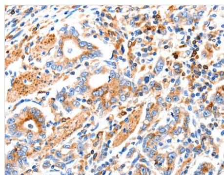
IHC (Immunohistochemistry) Immunohistochemistry of paraffin-embedded Human gastric cancer using MAP2K2 Polyclonal Antibody at dilution of 1:100
