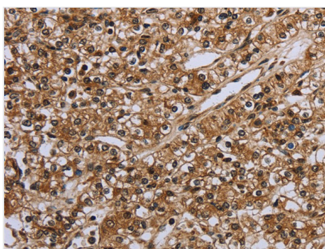
IHC (Immunohistochemistry) Immunohistochemistry of paraffin-embedded Human prostate cancer tissue using IL31RA Polyclonal Antibody at dilution 1:20
