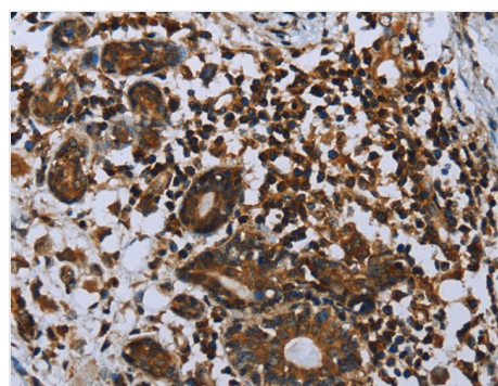
IHC (Immunohistochemistry) Immunohistochemistry of paraffin-embedded Human breast cancer tissue using IL31RA Polyclonal Antibody at dilution 1:20
