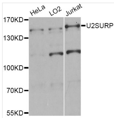
WB (Western Blot) Western blot analysis of extracts of various cell lines, using U2SURP Antibody.
