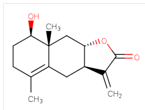
Structure 8-Epiivangustin, CAS 68776-48-7
