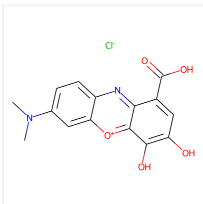
Structure Gallocyanine, CAS 1562-85-2
