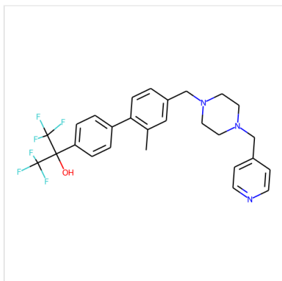
Structure SR 1903, CAS 1414248-06-8
