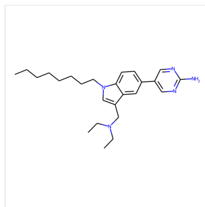
Structure CAY10677, CAS 1443253-20-0
