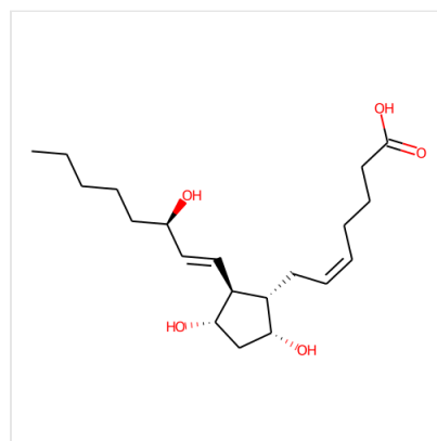
Structure ent-Prostaglandin F2alpha, CAS 54483-31-7
