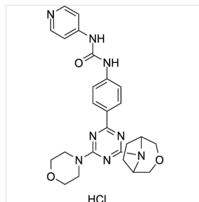
Structure PKI-179 hydrochloride, CAS 1463510-35-1
