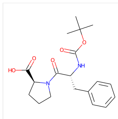
Structure Boc-D-Phe-Pro-OH, CAS 38675-10-4
