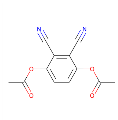
Structure 3,6-diacetoxy Phthalonitrile, CAS 83619-73-2
