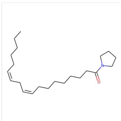
Structure Pyrrolidine Linoleamide, CAS 3140-51-0
