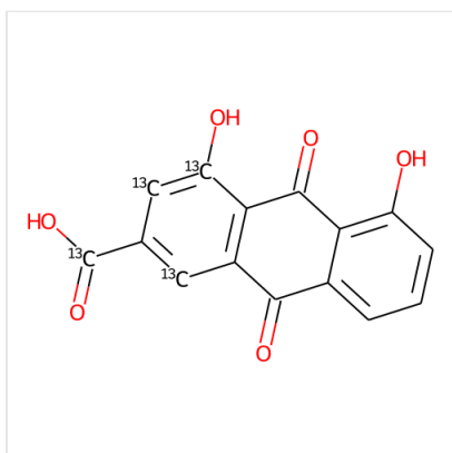
Structure Rhein-13C4, CAS 1189928-10-6
