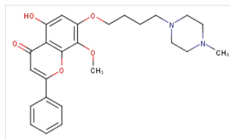
Structure LYG-202, CAS 1175077-25-4
