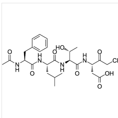
Structure Ac-FLTD-CMK, CAS 2376255-48-8
