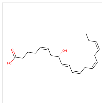
Structure 8(S)-HEPE, CAS 118492-81-2
