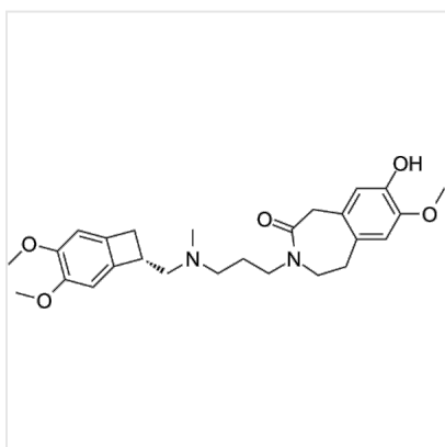
Structure 8-Demethyl Ivabradine, CAS 304464-97-9
