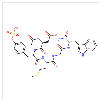
Structure CCK (26-30)(sulfated), CAS 89911-69-3
