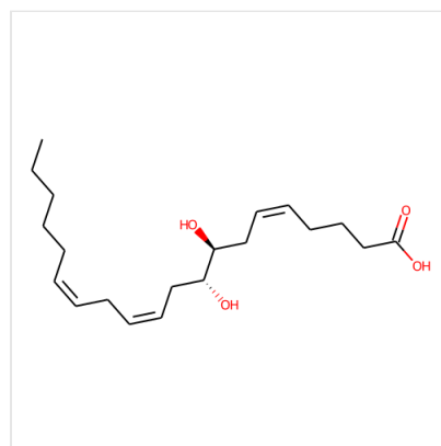
Structure +/-)-8(9)-DiHET, CAS 192461-96-4
