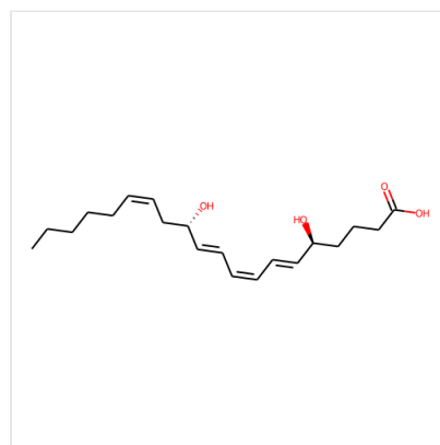
Structure 5(S),12(S)-DIHETE, CAS 79056-01-2
