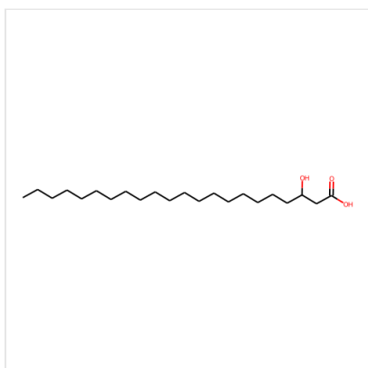
Structure 3-hydroxy Docosanoic Acid, CAS 89946-08-7
