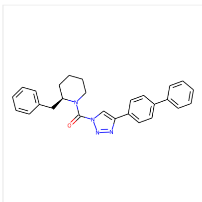
Structure R)-KT109, CAS 2055172-60-4
