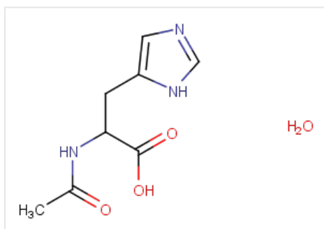
Structure N-Acetyl-L-histidine monohydrate, CAS 39145-52-3
