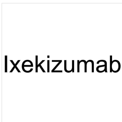
Structure Ixekizumab, CAS 1143503-69-8
