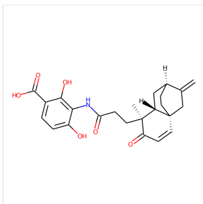
Structure Platencin, CAS 869898-86-2
