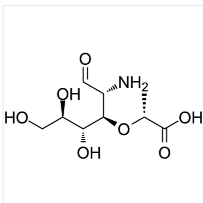
Structure Muramic acid, CAS 1114-41-6
