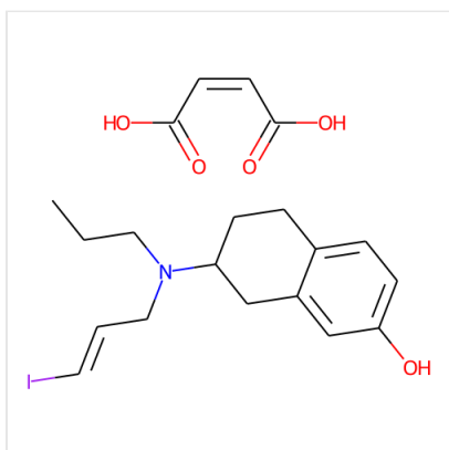
Structure 7-Hydroxy-PIPAT maleate, CAS 159559-71-4
