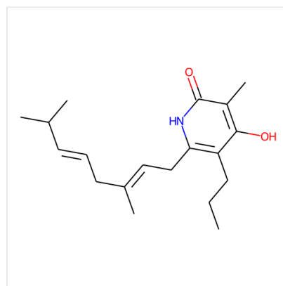
Structure Iromycin A, CAS 213137-53-2
