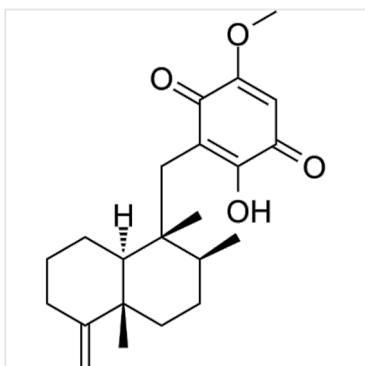
Structure Ilimaquinone, CAS 71678-03-0
