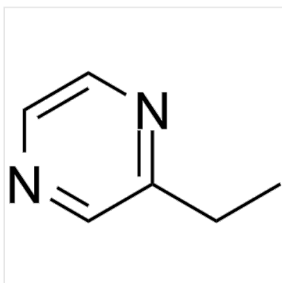
Structure 2-Ethylpyrazine, CAS 13925-00-3
