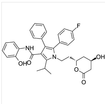
Structure 2-Hydroxy atorvastatin lactone, CAS 163217-74-1
