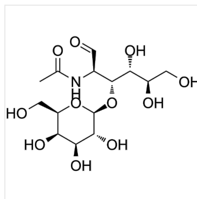
Structure Lacto-N-biose I, CAS 50787-09-2
