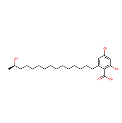
Structure Phanerosporic Acid, CAS 124709-28-0
