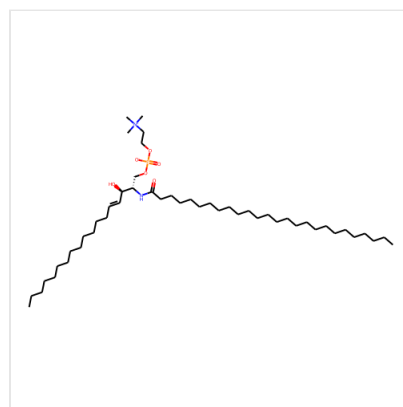
Structure C26 Sphingomyelin (d18:1/26:0), CAS 221097-57-0
