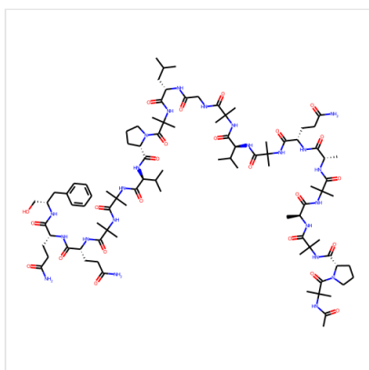
Structure Alamethicin F50, CAS 56165-93-6
