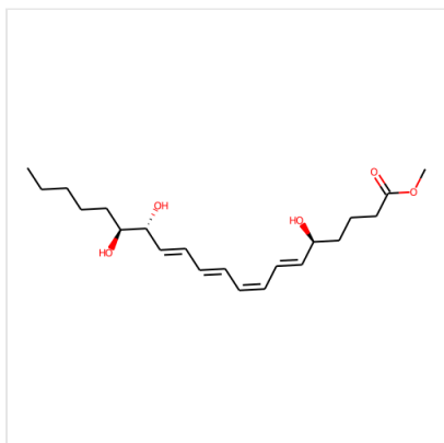
Structure Lipoxin B4 methyl ester, CAS 97589-07-6
