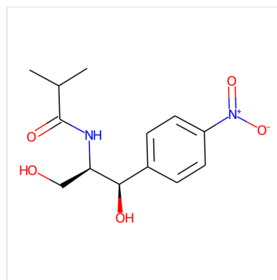
Structure Corynecin III, CAS 18048-95-8
