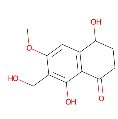
Structure 10-Norparvulenone, CAS 618104-32-8
