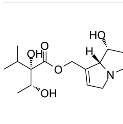
Structure +)-Intermedine, CAS 10285-06-0
