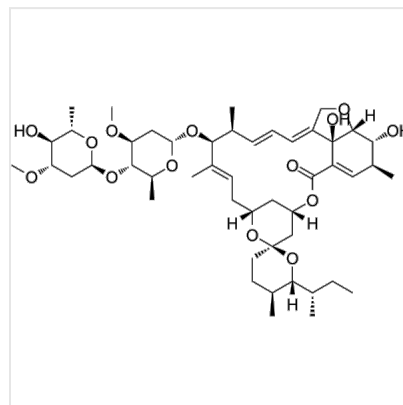
Structure 2,3-Dehydro-3,4-dihydro ivermectin, CAS 1135339-49-9
