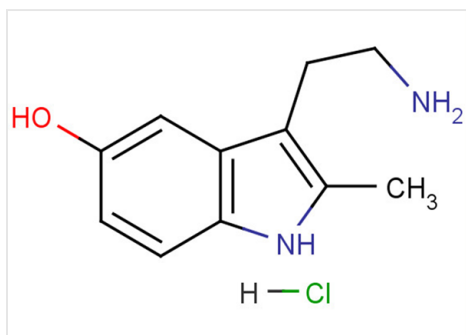
Structure 2-Methyl-5-HT hydrochloride, CAS 845861-49-6
