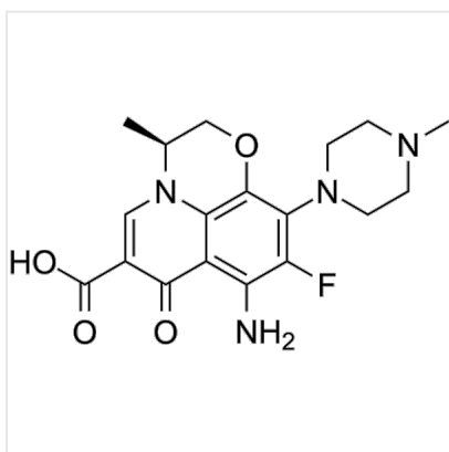
Structure Antofloxacin, CAS 119354-43-7
